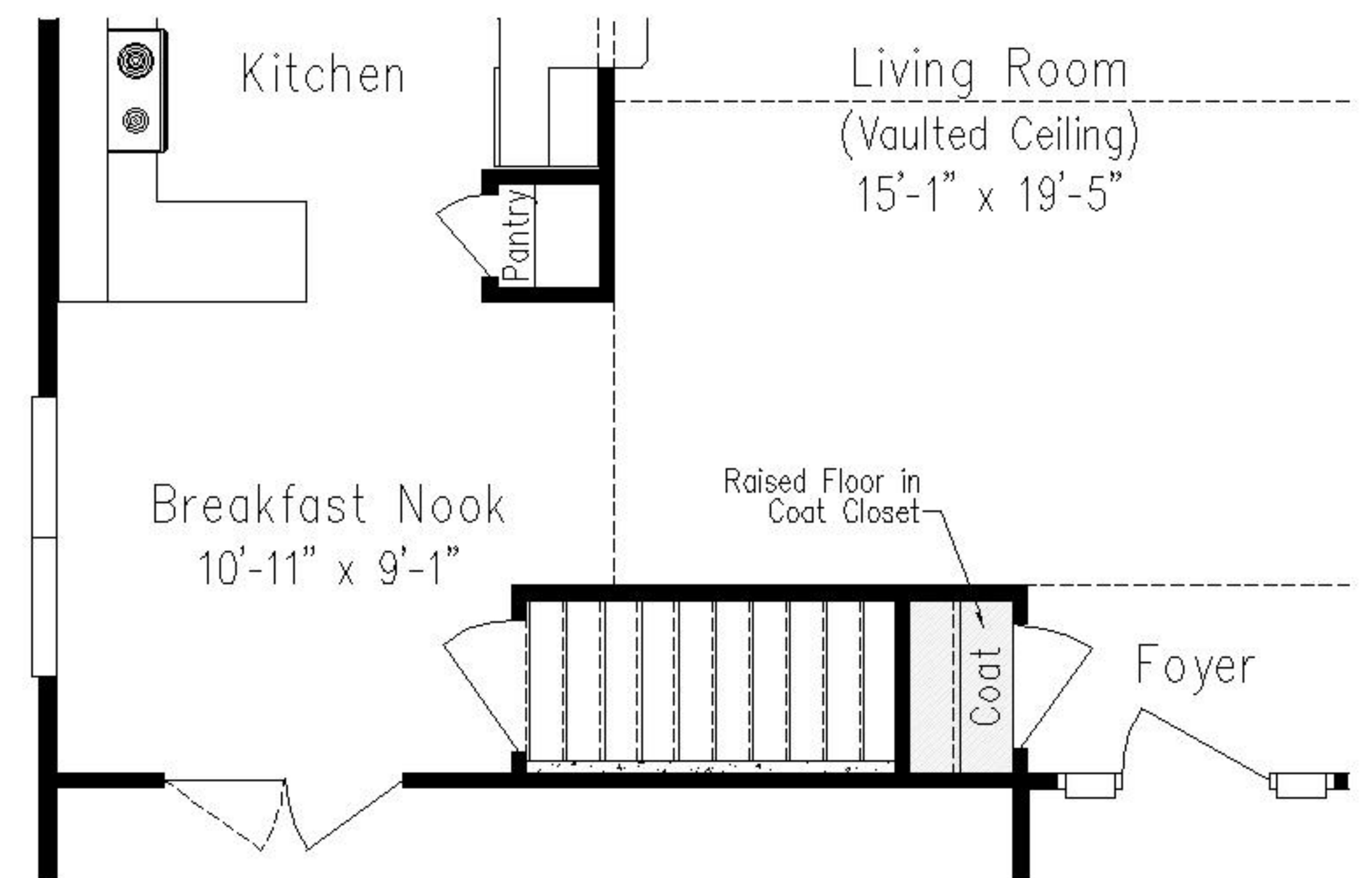
Partial Floor Plan with Optional Basement Stairs
