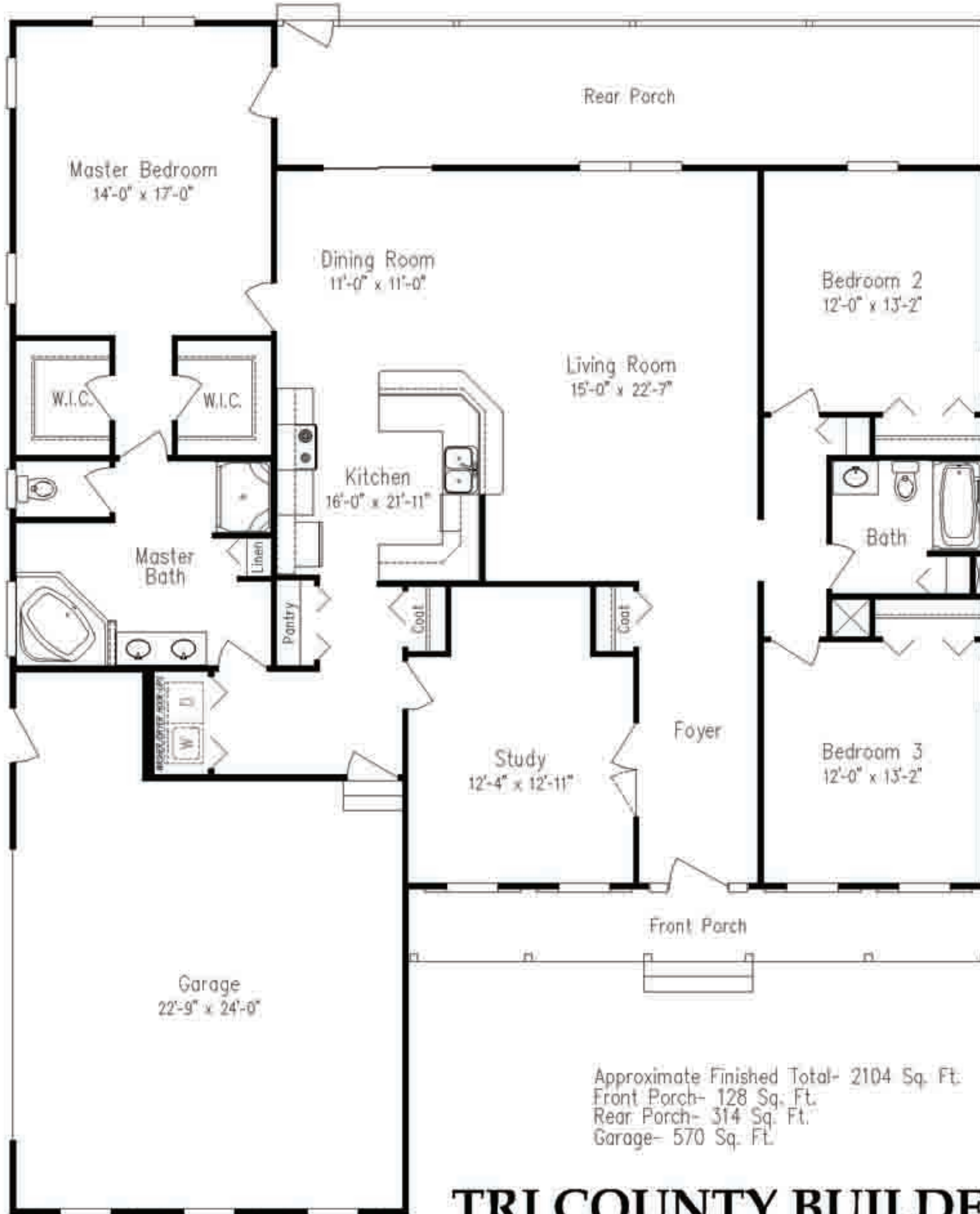
Floor Plan
