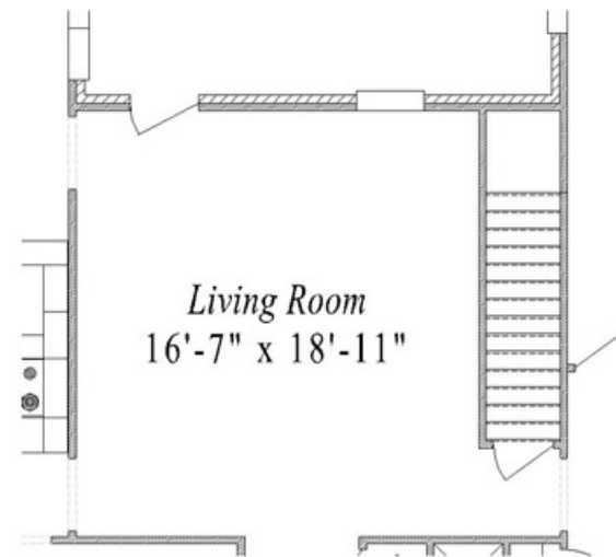
Partial Floor Plan with Basement Stairs
